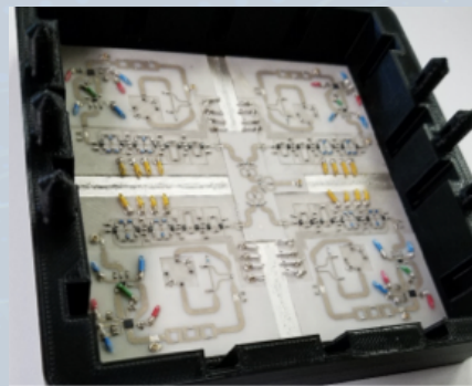
3d Printed Flat Shape (single/multi layer PCB)
