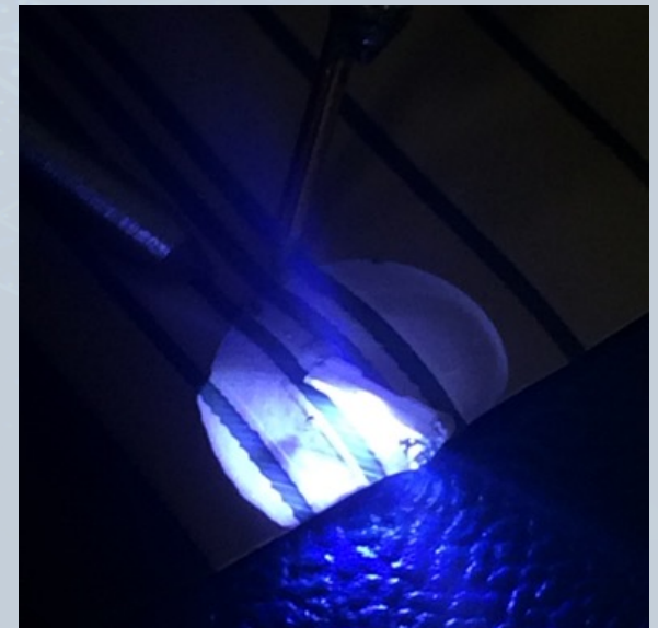
3d Printed Flexible Shape (PCB) + Rigid Hybrid Electronics
